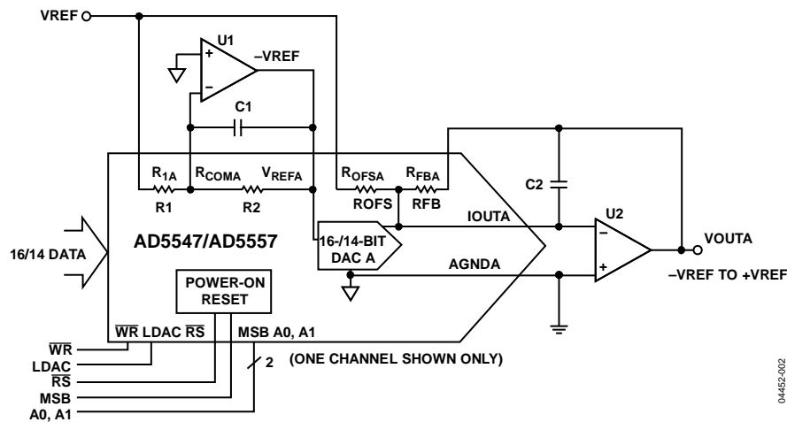
Figure 2. 16-/14-Bit 4-Quadrant Multiplying DAC with Minimum of External Components (Only One Channel Is Shown)
