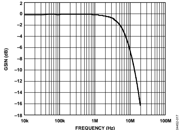
Figure 16. AD5547 Unipolar Reference Multiplying Bandwidth
