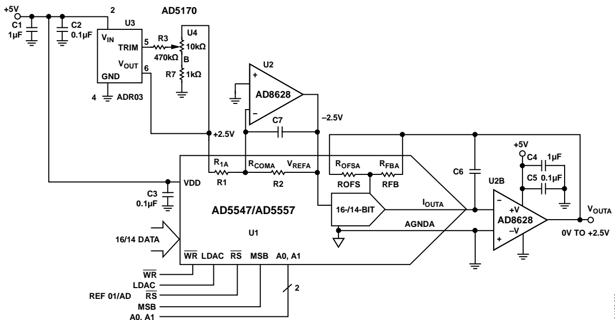
Figure 24. Full-Span Calibration
