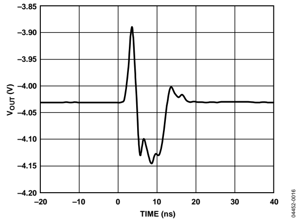
Figure 15. AD5547 Midscale Transition and Digital Feedthrough
